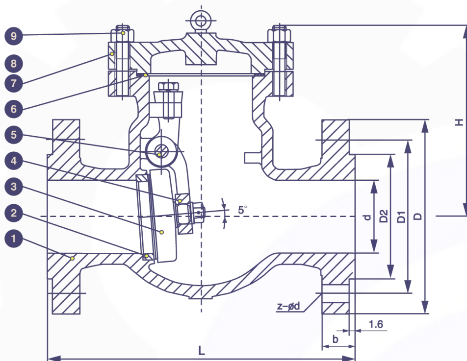
ANSI 150# Cast Steel Flange End Swing Check Valves
