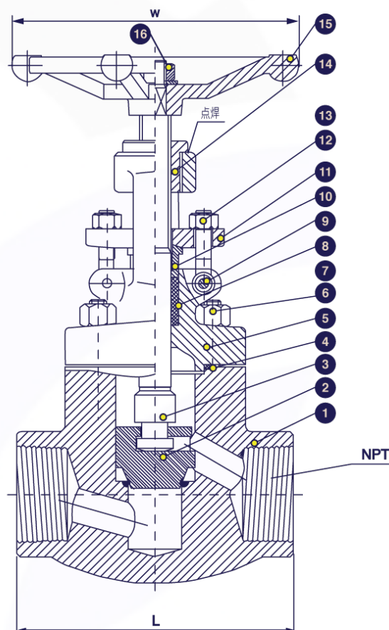
Threaded End SS316 Globe Valves 800 PSI
