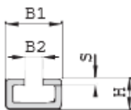
Mounting Rail
