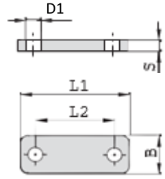
Cover Plate
