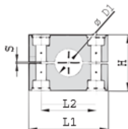
Clamp Body
