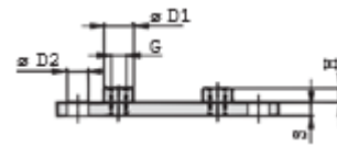
Elongated Weld Plate
