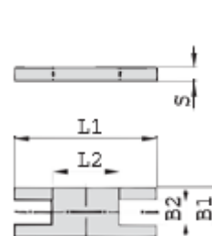
Safety Locking Plate
