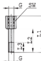
Stacking Bolt
