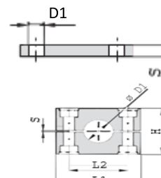
Cover Plate
