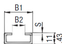
Mounting Rail
