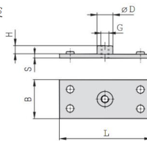
Weld Plate
