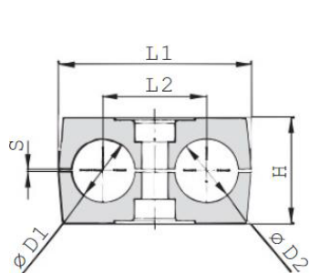
Clamp Body
