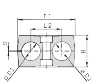
Clamp Body
