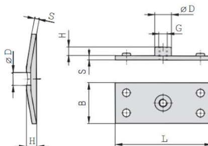
Cover Plate
