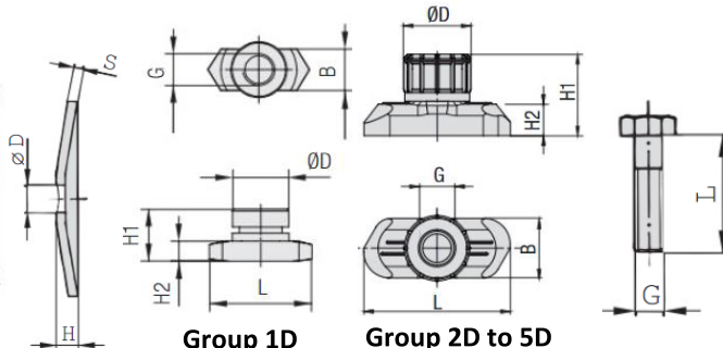
Rail Nut
